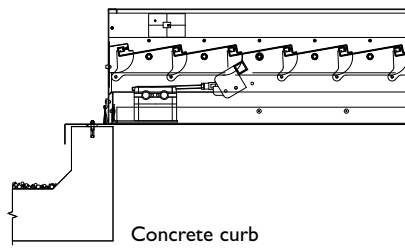
TYPICAL BASE DETAIL FOR CURBS
